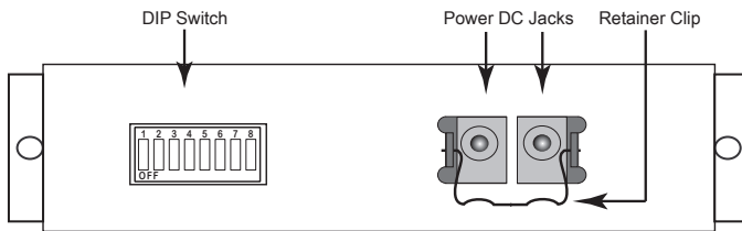
Figure 3: Rear Panel AC (external transformer "brick") power models
