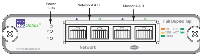
Figure 2: Front Panel, 10/100/1000BaseT Taps (TP-CU3, TP-CU3-DC)
