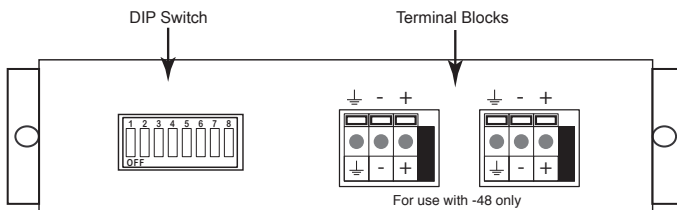
Figure 5: Rear Panel DC power model TP-CU3-ZD-DC
