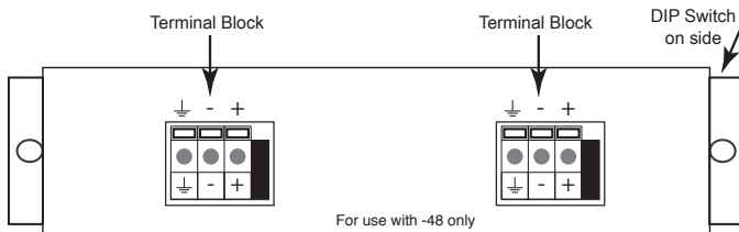
Figure 4: Rear Panel DC power model TP-CU3-DC
