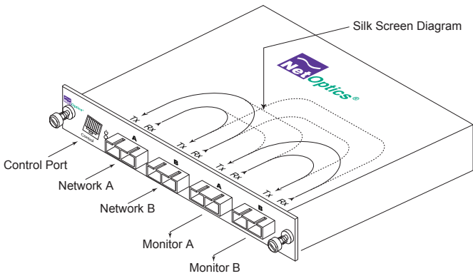
Figure 2. BPO-SX-1 and BPO-LX-1 models with RJ45 port
